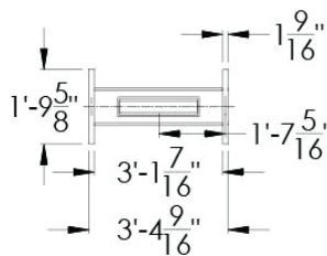
6' TABLE BASE
