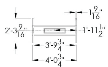
4' EXT TABLE BASE
