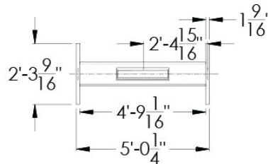
8', 10', 12' TABLE BASE
